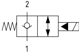
Hydraulic diagram
