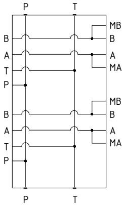
Hydraulic diagram
