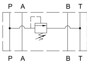
Hydraulic diagram
