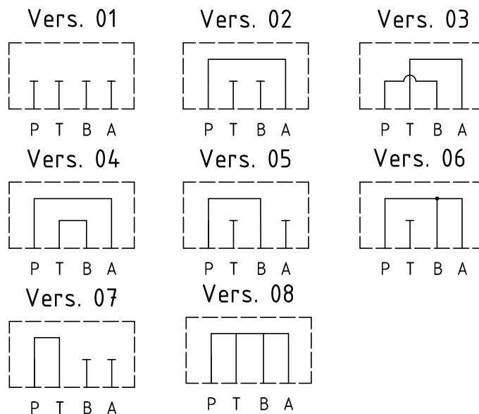
Hydraulic diagram
